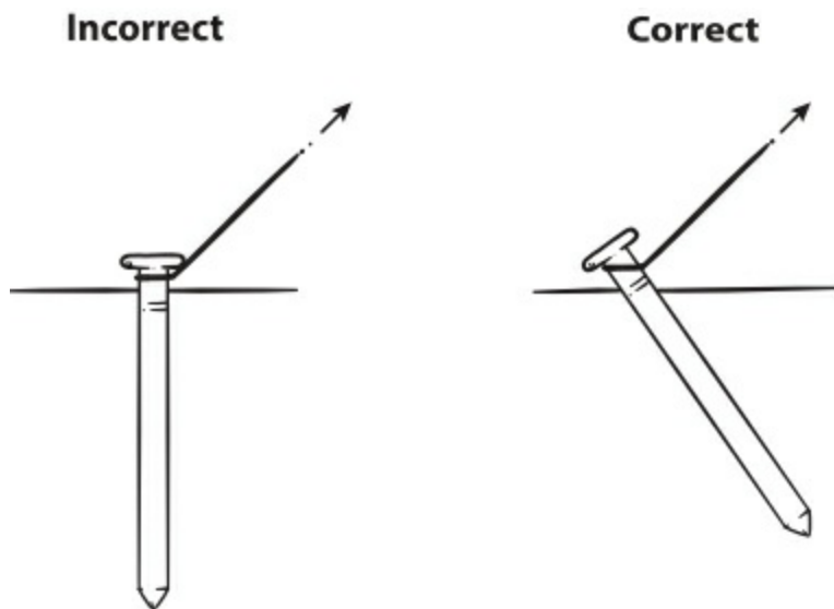
Stake-driving angles
