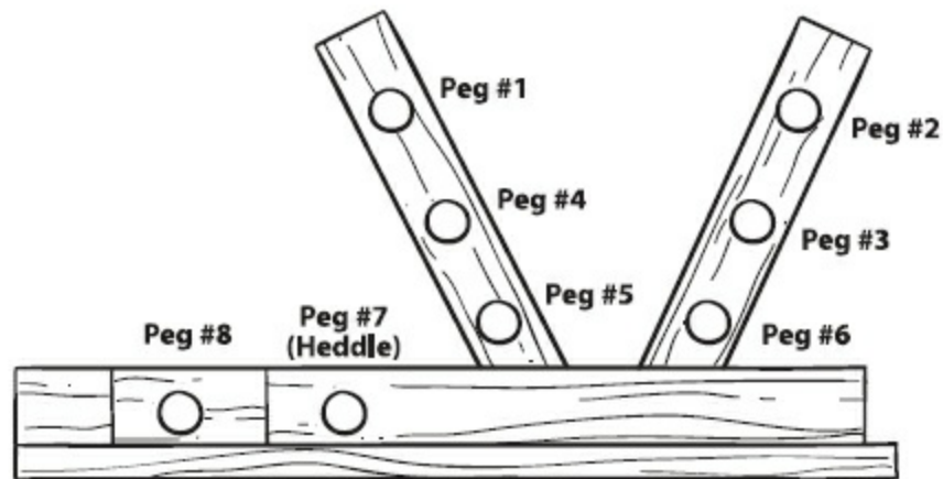
Inkle loom
