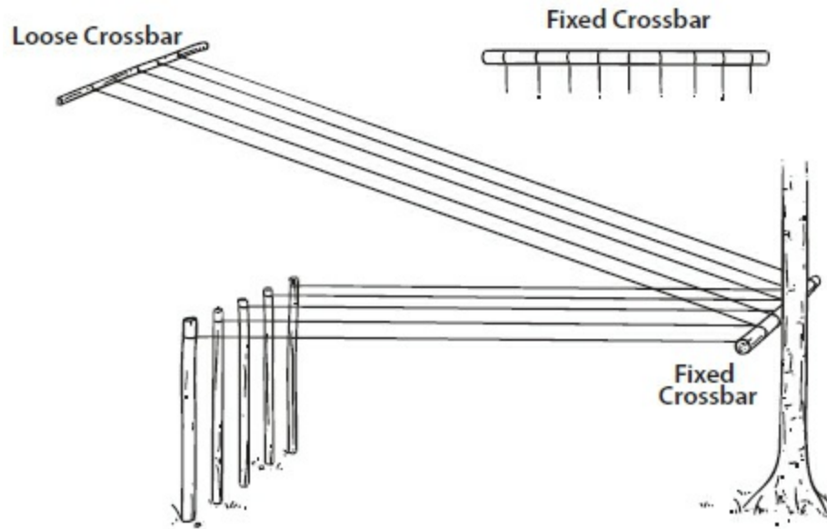
Woodland loom
